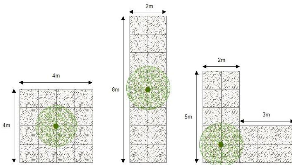
Figure 35. Typical tree pit arrangements for medium sized trees | DCC
